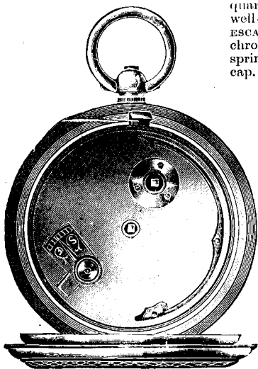
Illustration showing Dust proof Cap as fitted to the "SUPER-GREENWICH" Lever.
